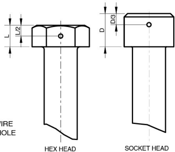
FIGURE 3. DRILLED HOLE LOCATION
